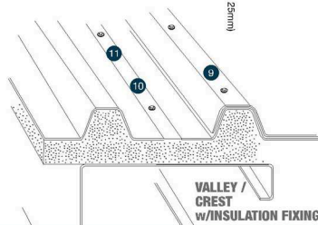
VALLEY FIXING FOR THICK STEEL
