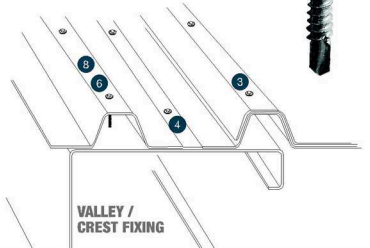
VALLEY / CREST w/INSULATION FIXING
